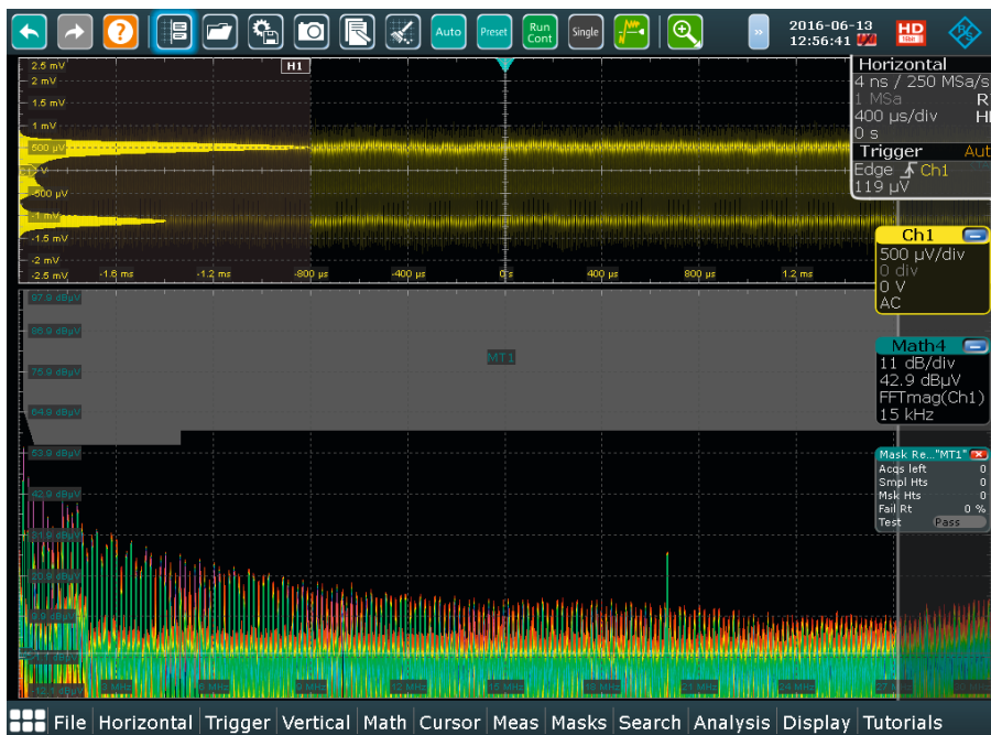
Mask test in the frequency domain.
